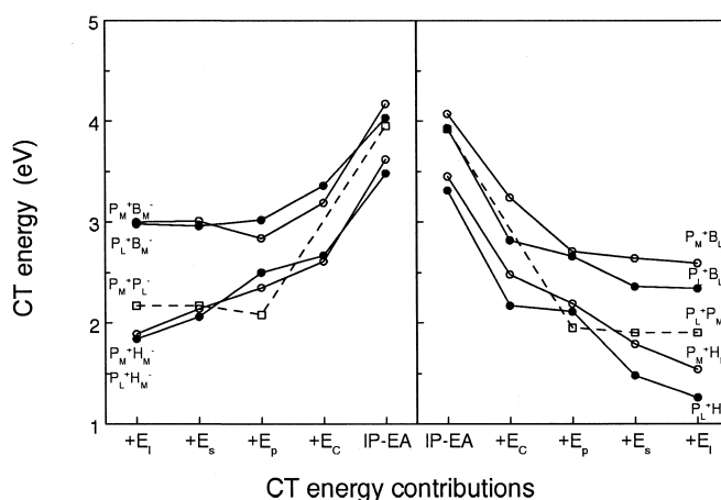
Fig. 3 The calculated energies of the charge transfer states are shown. Several contributions are presented separately. Ionisation potentials of the donor IP and electron affinities of the acceptor EA are estimated from the calculated MO energies of the isolated chromophores. The Coulomb energy E_c results from the corresponding electron densities of the MO's. The polarization contribution E_p is evaluated from a calculation including the six chromophores as a supermolecule. Short range interactions E_s refer to the residues shown in Fig. 1 and are treated explicitly whereas long range electrostatic effects E_L are treated in a continuum approximation
