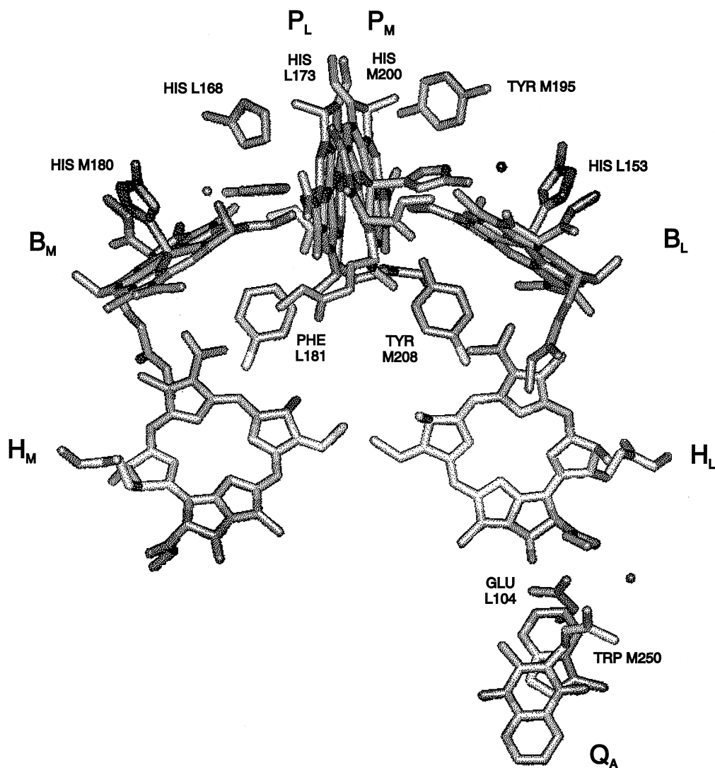
Fig. 1 The quantum chemically treated part of the reaction center Rps. viridis is shown. It consists of the four bacteriochlorophylls B_M , P_L , P_M and B_L , the two bacteriopheophytins H_M and H_L , the quinon Q_A and several protein residues which are in close contact
