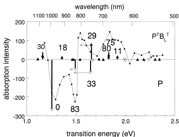
Fig. 4 The calculated transient difference spectrum of P^T B_L^T (bars) is compared with experimental values (circles) from (Dressler et al. 1990). The numbers show the calculated polarization angles relative to the dimer band P^* . The horizontal arrows, indicate the energy shifts needed for the experimental assignment
