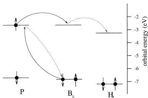
Fig. 2 The electron assisted electron transfer mechanism is visualized. The solid arrows refer to the initial presumably slower (3.5 ps) fission process P^* \rightarrow P^+ B_L^- , which invokes a two electron exchange between P and B_L . The dashed arrows give the second faster (0.65 ps) charge separating step as a simultaneous transfer of an electron from B_L to H_L and one from P to B_L . The orbital energies refer to the neutral ground state of the hexamer from Fig. 1
